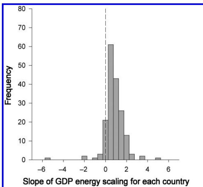
Figure 2. The frequency distribution of exponents (slopes from log-log plots) of economic trajectories of per capita energy use as a function of per capita gross domestic product (GDP) within countries over the time series from 1980 to 2003. The average slope is approximately 0.6 and nearly all countries showed positive growth over the 24-year period. Source: Data are from the World Resources Institute ( http://earthtrends.wri.org/index.php ) and the International Energy Agency ( www.iea.org/stats/index.asp ).
