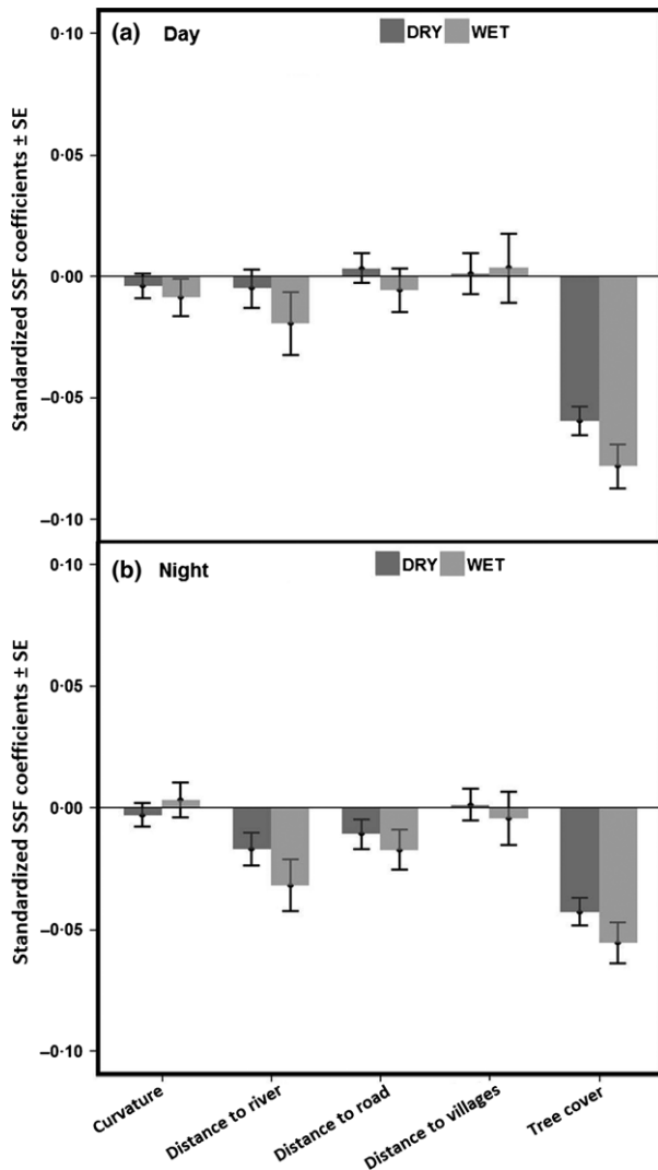
Fig. 2. Step selection function (SSF) coefficients for the strength of avoidance of landscape variables in (a) day and (b) night by hirola during dry and wet seasons. Note that 'river', 'road', and 'villages' are distance variables, such that a negative coefficient indicates selection for the corresponding variable.
